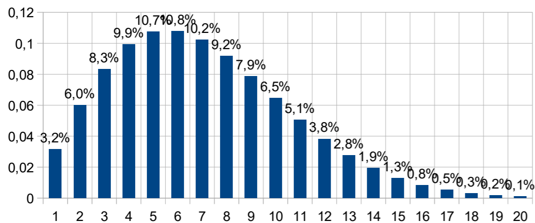
Annual Energy 5175 kWh - with average wind speed 6m/s
