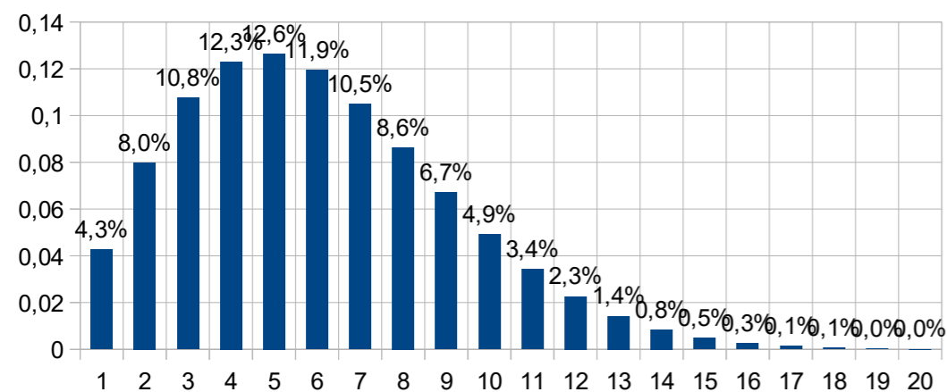
Annual Energy 5175 kWh - with average wind speed 6m/s
