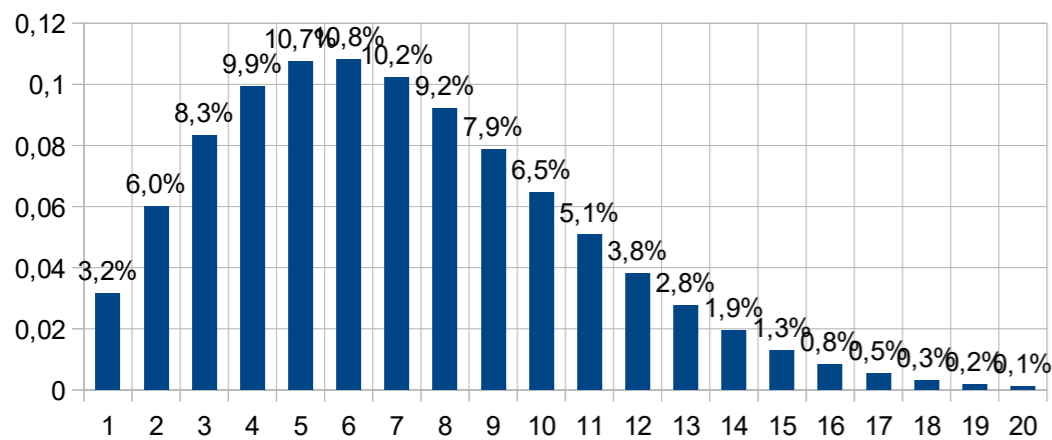
Annual Energy 1393 kWh - with average wind speed 6m/s
