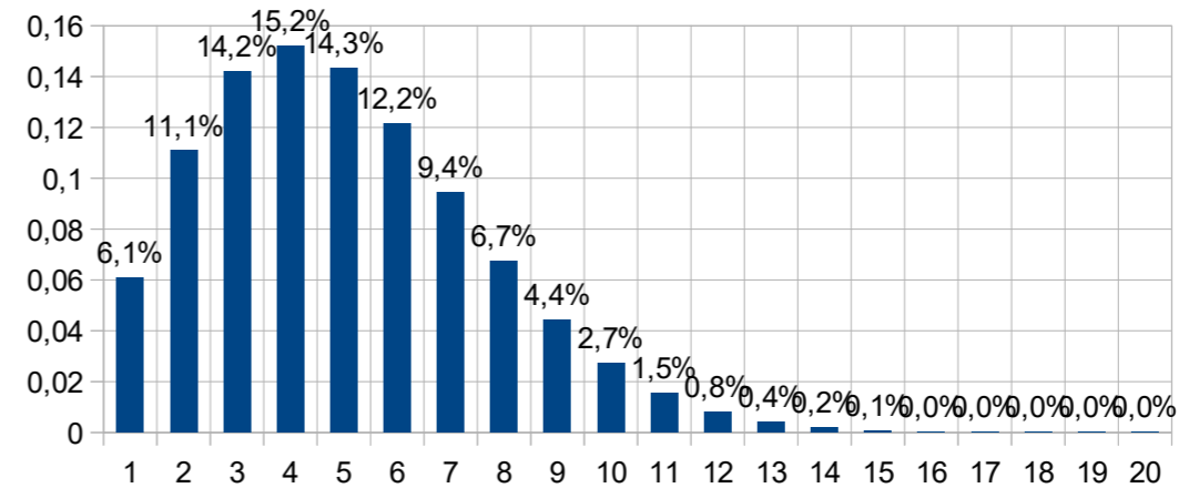
Annual Energy 488 kWh - with average wind speed 4m/s
