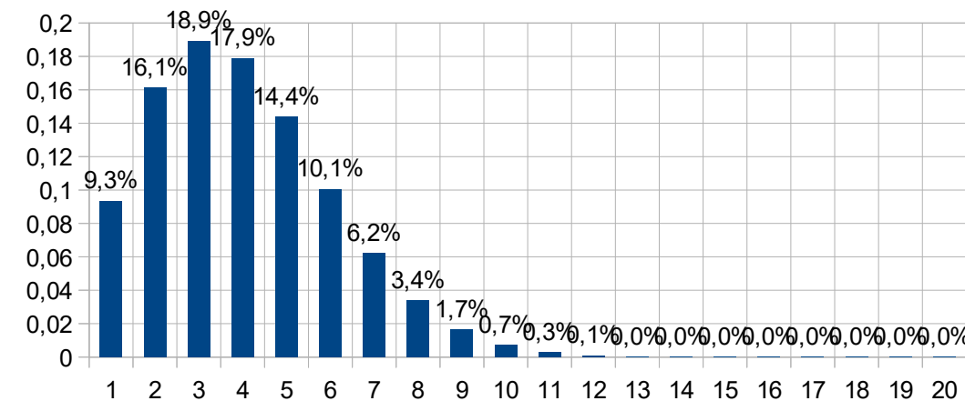
Annual Energy 736 kWh - with average wind speed 4m/s
