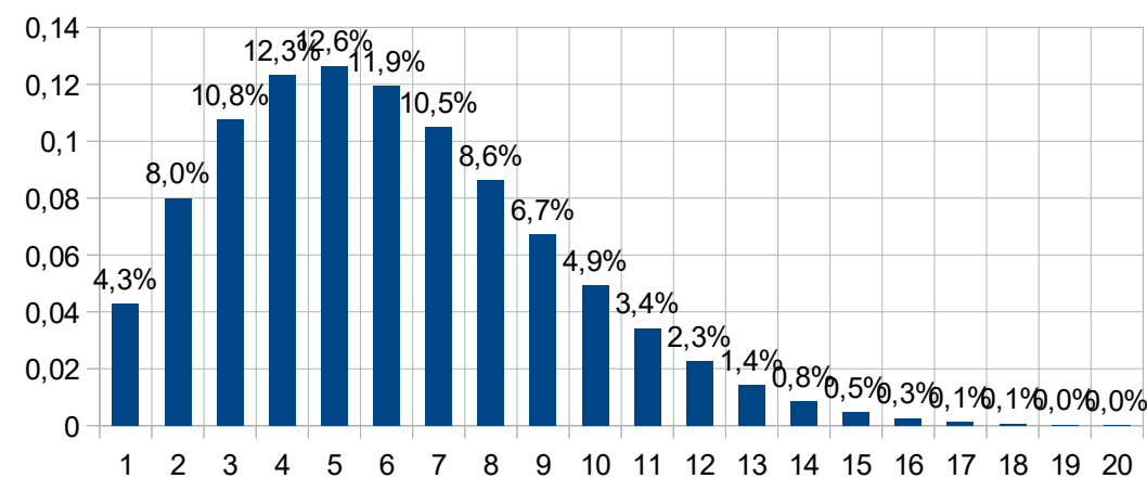
Annual Energy 2347 kWh - with average wind speed 6m/s
