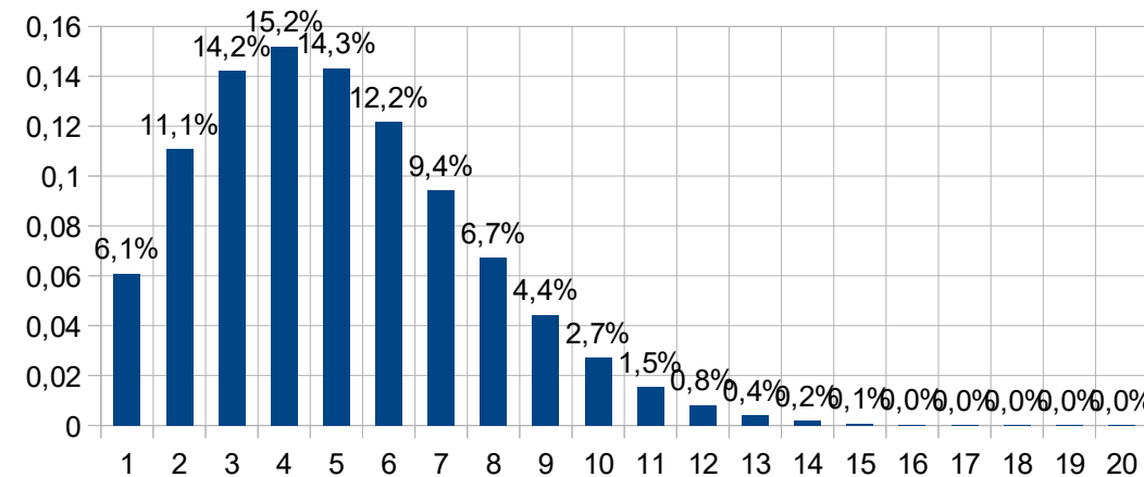
Annual Energy 736 kWh - with average wind speed 4m/s
