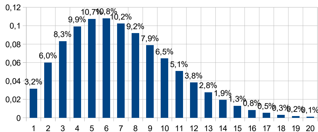
Annual Energy 2347 kWh - with average wind speed 6m/s
