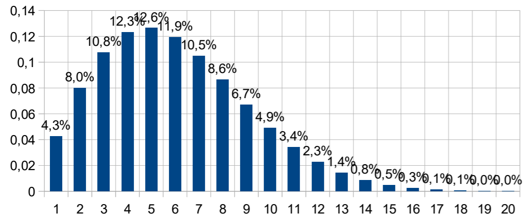
Annual Energy 7125 kWh - with average wind speed 6m/s
