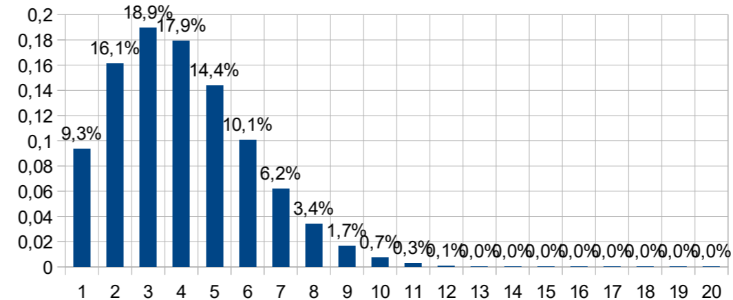
Annual Energy 2324 kWh - with average wind speed 4m/s
