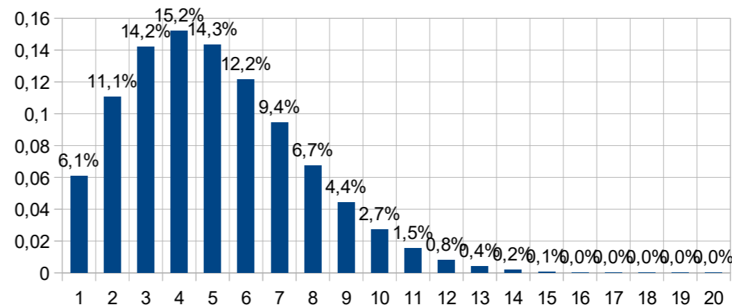
Annual Energy 2324 kWh - with average wind speed 4m/s
